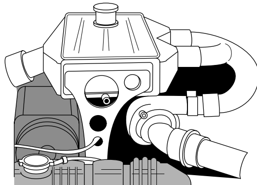
Figure 18-1: An air-to-water intercooler installed on a turbocharged engine.
