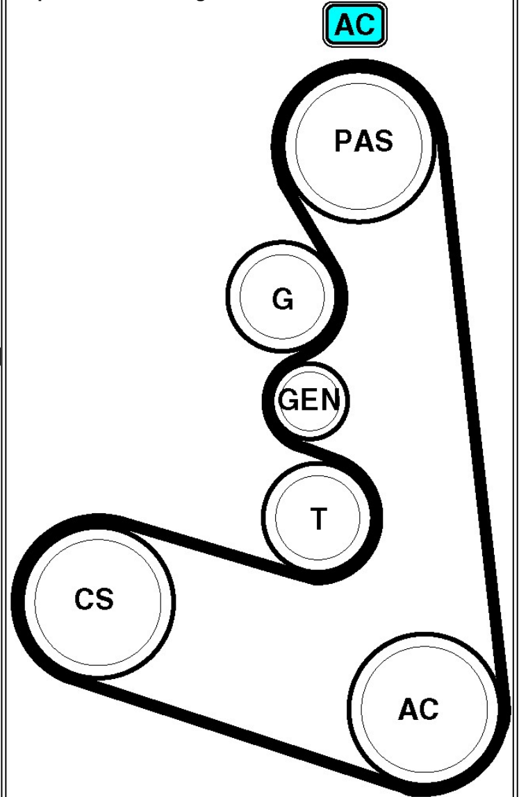
Serpentine belt routing
