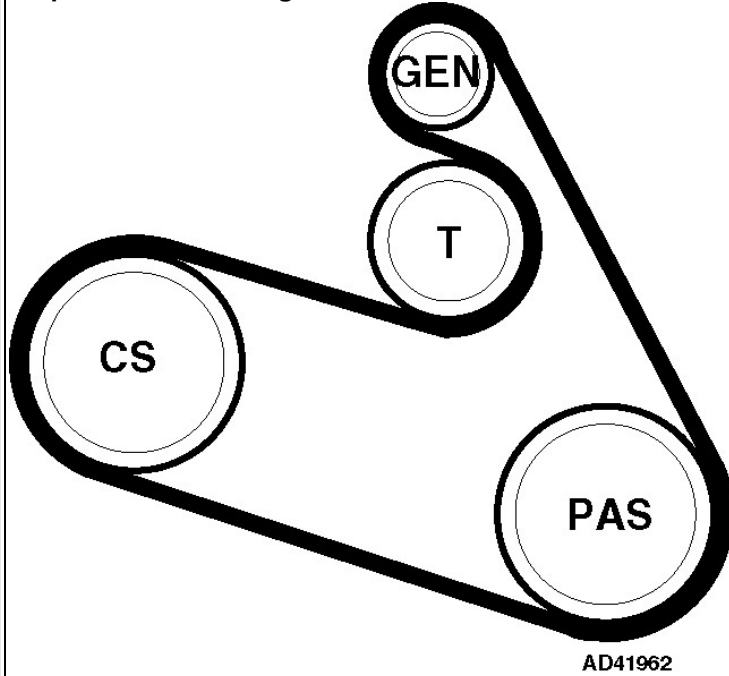
Serpentine belt routing
